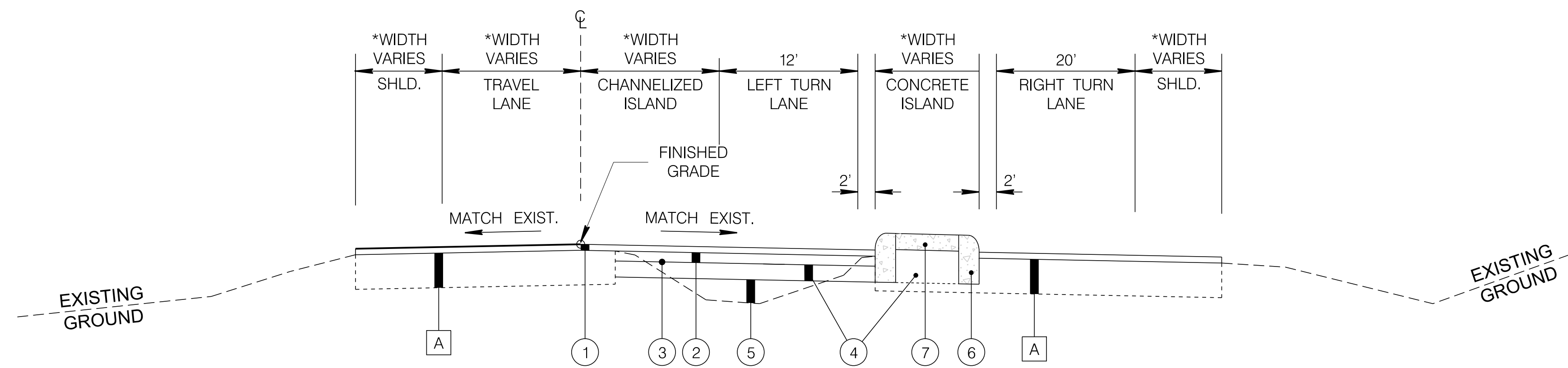
CLAYTON ARNOLD ROAD TYPICAL SECTION
